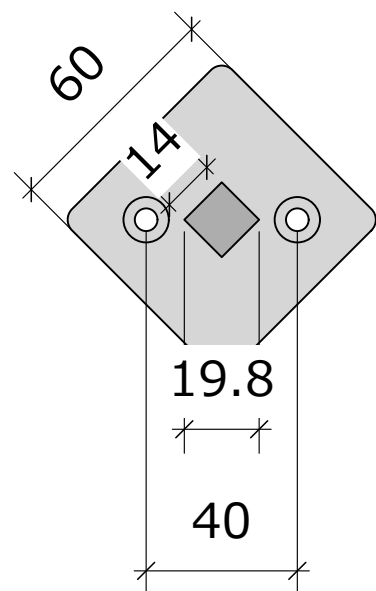
台座60 x 60mm | T5mm Φ6 x 12皿穴
